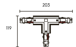
T connector left 2 DALI 3 circuit
