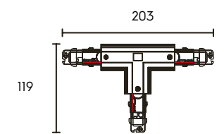
T connector right 2 DALI 3 circuit
