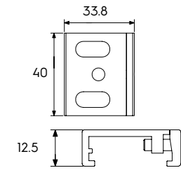
Fixed monopoint for track adapter
