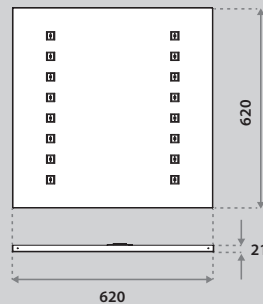
Aviora FL 2L 620x620 (IP20)
