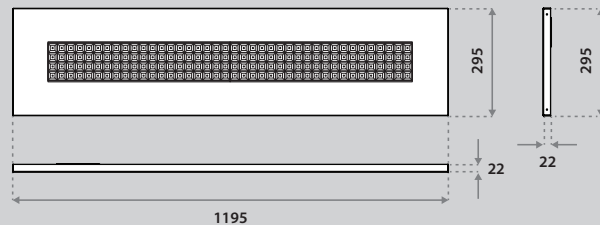
Linessa 2L 1195x295 (IP20)
