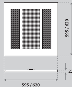
Linessa Air 595x595 / 620x620 (IP20)
