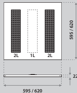
Linessa 2L 595x595 / 620x620 (IP20)
